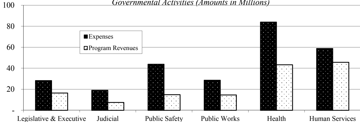
Graph 1 Expenses and Program Revenues Governmental Activities (Amounts in Millions)
